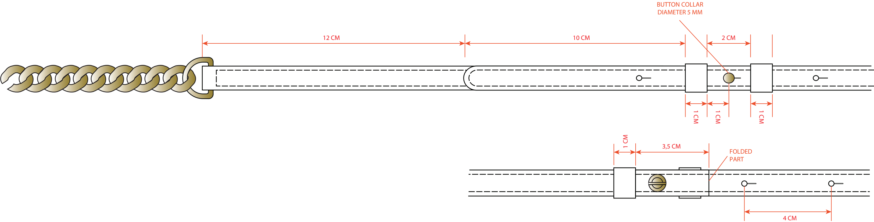
BOTTOM VIEW OF SHOULDER STRAP ADJUSTMENT
